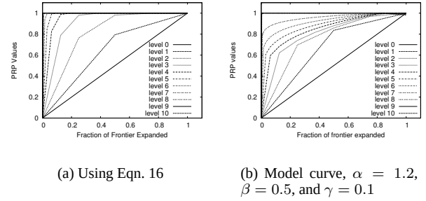
Figure 4. PRP values for uniform binary search tree
