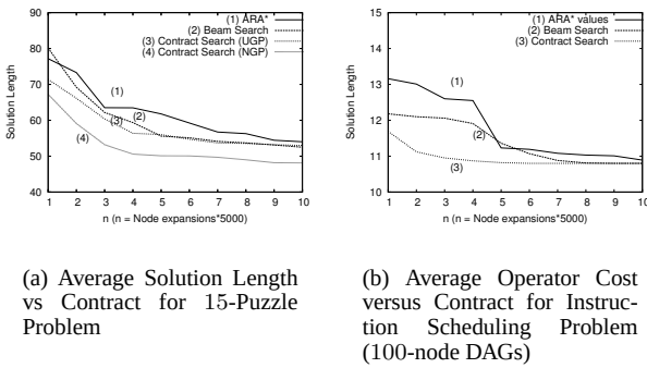
Figure 6. Comparative results for 15-Puzzle and Instruction Scheduling: ARA*, beam search, and Contract Search.
