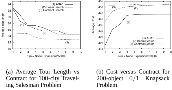
Figure 5. Comparative results for TSP and 0/1 Knapsack: ARA*, beam search, and Contract Search.
