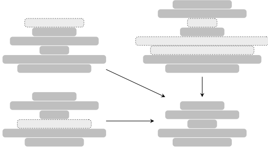
Figure 5. Size-independence and symmetric lookups for relative-order abstractions: three different abstractions map to the same state in S_5 .
