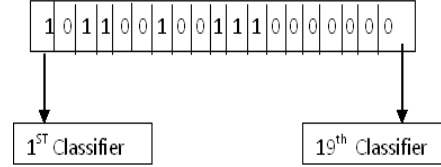
Figure 1. Chromosome Representation
