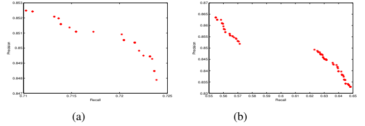
Figure 2. Pareto optimal front for (a) Bengali (b) Hindi
