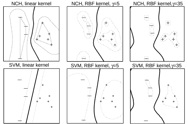
Figure 4. Decision boundaries for NCH and SVM using the linear and RBF kernels on a linearly separable data set. The dashed contours for the NCH method are iso-curves along which the ratio of the distances to the two convex hulls is constant.
