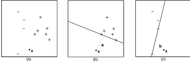
Figure 3. Classification of a test point \mathbf{x} with NCH on the binary data set in Panel (a) in two steps. At stage one (Panel (b)), a test point \mathbf{x} is added to a data set that contains only the positive class, and the distance \mathbf{a} from \mathbf{x} to the convex hull of this class is computed. At stage two (Panel (c)), \mathbf{x} is added to a data set that contains only the negative class, and the distance \mathbf{b} from \mathbf{x} to the convex hull of this class is computed. If \mathbf{a} > \mathbf{b} ( \mathbf{a} < \mathbf{b} ), then \mathbf{x} is assigned to the negative (positive) class.
