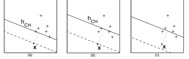
Figure 2. Classification of a test point \mathbf{x} with (hard) NCH in Panel (a), soft NCH in Panel (b), and soft SVM in Panel (c). In Panel (b), the hyperplane from Panel (a) is “pushed” further away from \mathbf{x} and inside the convex hull of the positive class, resulting in a soft distance from \mathbf{x} to this convex hull. In Panel (c), the distance between the two parallel hyperplanes represents the so-called (twice) SVM margin. In this case the slack is applied to both \mathbf{x} and the points from the positive class, unlike the soft NCH, where no slack is applied to \mathbf{x} .
