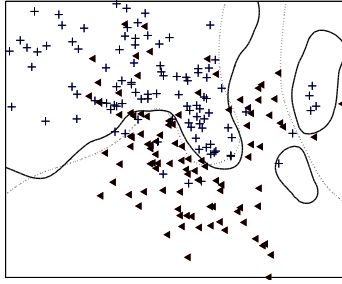
Figure 5. The NCH-optimal (using the RBF kernel) decision boundary found using a leave-one-out cross-validation procedure for tuning the C and \gamma parameters in solid contour and Bayes-optimal decision boundary in dashed contour on a synthetic data set introduced in [11]. The Bayes error is 0.210, and the test error of the NCH classifier is 0.228. The instances of the two classes are denoted with pluses and triangles. The data set is balanced and consists of 200 instances in total.
