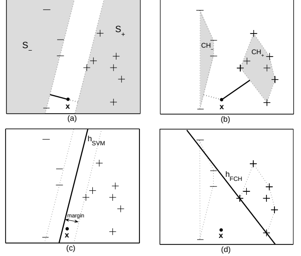
Figure 1. Classification of a test point \mathbf{x} with SVM in Panels (a) and (c), and NCH in Panels (b) and (d) on a binary data set. In Panel (a), the white band has the largest possible width, which is equal to twice the margin, shown in Panel (c). The points to the left and to the right of the band form shaded sets S_- and S_+ , respectively. Test point \mathbf{x} receives label +1 since it is farther from S_- than S_+ . In Panel (b) point \mathbf{x} is classified as -1 since it is farther from the convex hull of the positive points, CH_+ , than from the convex hull of the negative points, CH_- .
