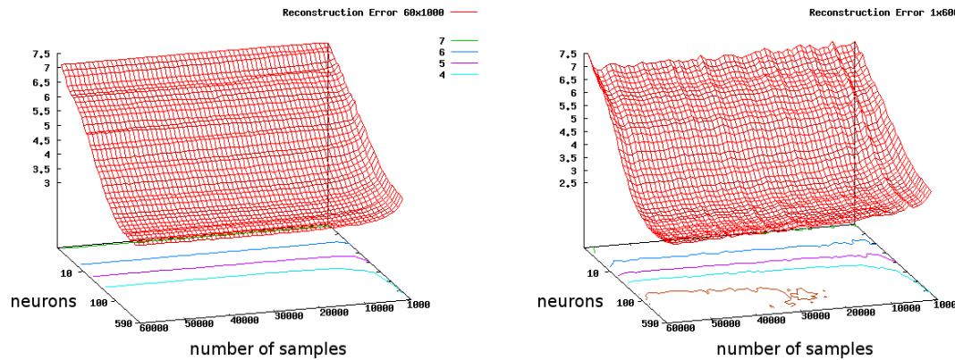
Figure 11. Reconstruction Error for RBM trained on 60x1,000 (Left) and 1x60,000 examples (Right) as a function of the number of neurons and gradient updates.
