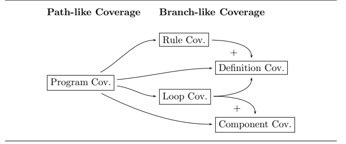
Figure 1. Relations between total coverage of different notions.
