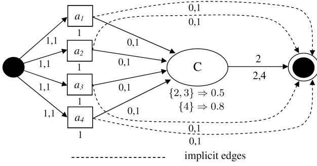
Figure 2: The CF-NET representation of Example 1.
