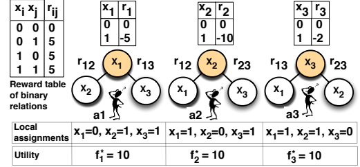
Figure 1. Example of an initial division in a 3 agent DCOP.
