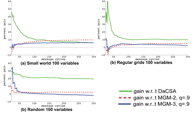
Figure 2. Percent gain of EU-DaC with respect to DaCSA and MGM-{2,3}
