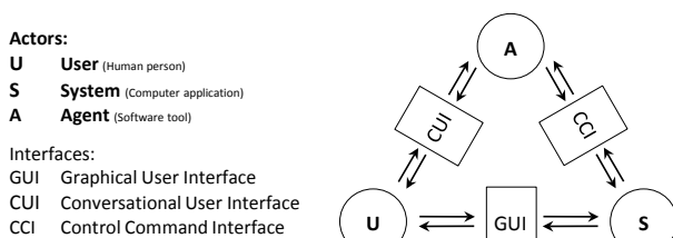
Figure 1. A typical Assistant Conversational Agent architecture
