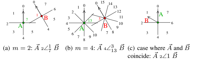
Figure 1. Two oriented points related at different granularities.
