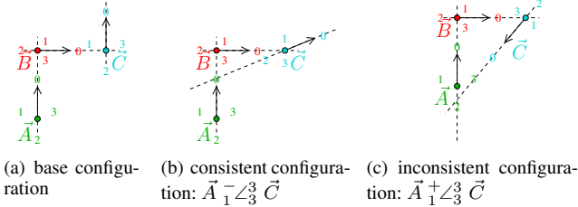
Figure 2. Examples of bipath composition results for \mathcal{OPRA}_m^* relations \vec{A} \perp \angle_0^3 \vec{B} and \vec{B} \perp \angle_0^1 \vec{C} .
