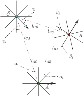
Figure 3. An exemplary triangle configuration for \vec{A} \frac{x}{m\angle_i^j} \vec{B} , \vec{B} \frac{y}{m\angle_k^l} \vec{C} , and \vec{A} \frac{z}{m\angle_t^s} \vec{C} .
