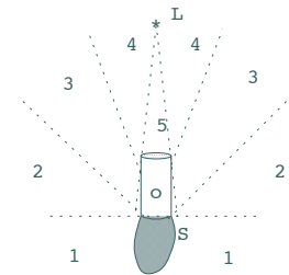
Figure 1. Regions implied by the observation of a shadow and its caster.
