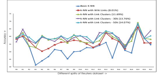
Figure 1. Effects of k -NN with m(=30k, =50k) Wiki hyperlink clusters
