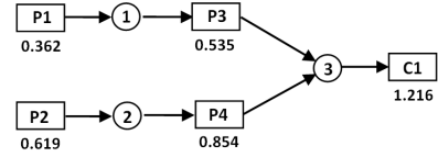
Figure 1. A sample supply chain network, from [3]. Producers (P1,P2,P3,P4) and consumers (C1) are represented by rectangles, with goods represented by circles. Edges between vertices show possible flows of goods. Numbers below producers indicate production costs, while numbers below consumers indicate consumption values.
