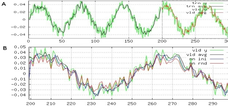
Figure 2. Output of the proposed ( nn_{ini} ) and standard ( nn_{rnd} ) models when compared with series input ( trn/vld_y ) and corresponding moving average ( trn/vld_y avg ). Subplot A presents train and test set, while subplot B zooms on test set.
