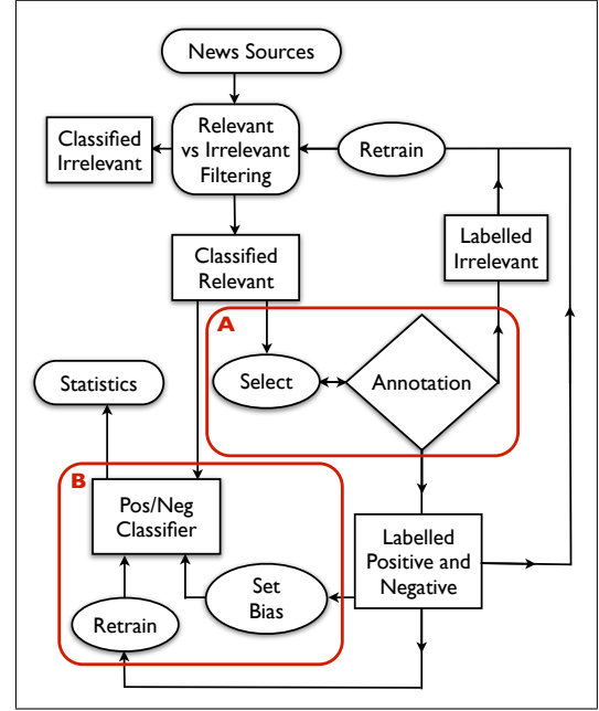
Figure 2. Overall design of the economic sentiment analysis system. The important components are (A) the article selection and annotation process, and (B) the training of the classifier where classification bias is controlled.
