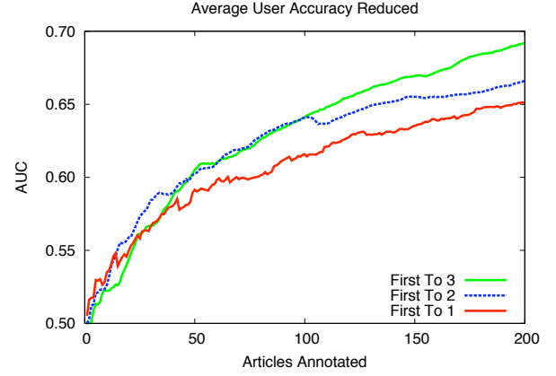
Figure 7. When reducing average annotator-majority agreement to 67%, coverage is still important in the early stages of the learning curve. By acquiring more annotations per article, consensus can be attained and, if a sufficient budget is available, classification performance can be improved.
