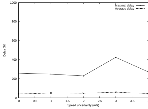
Figure 10. Average and maximal delays according to speed uncertainty.
