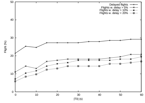
Figure 7. Number of delayed flights according to the initial time uncertainty.
