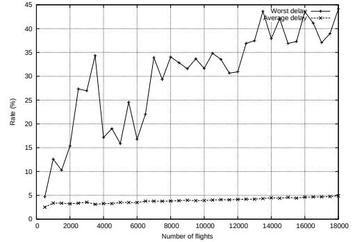
Figure 3. Relative average and worst delays.
