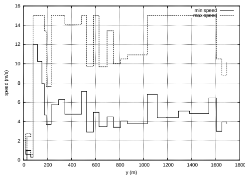
Figure 6. Speed bounds for flight 988 along its trajectory.
