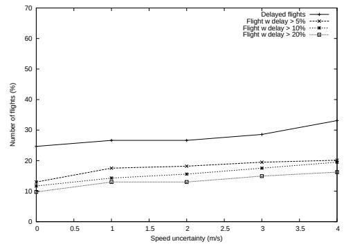
Figure 9. Number of delayed flights according to speed uncertainty.
