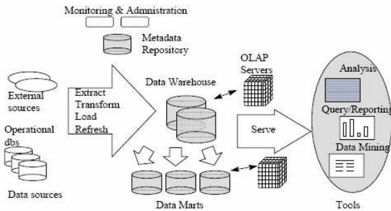
Figure 1. Architecture of a generic data warehouse system
