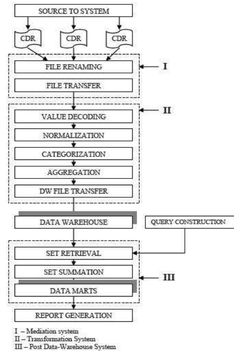
Figure 2. Report generation system based on call data
