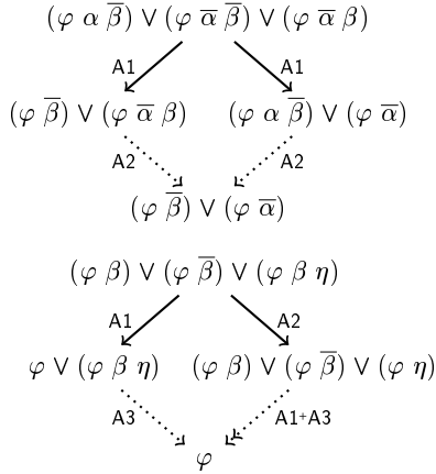
Figure 5. Examples of why the absorption rules A2 and A3 are needed. The conjunction sign \wedge has been omitted to save space. A1 necessitates the inclusion of A2, which again necessitates the inclusion of A3.
