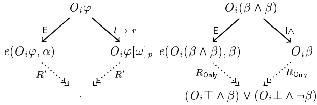
Figure 3. Left: Lemma 8: R' = R \cup \{l \rightarrow r\} -joinability is guaranteed as long as l \rightarrow r satisfies R -substitutional joinability and R_{\text{Min}} \subseteq R . Right: e(O_i(\beta \wedge \beta), \beta) and O_i\beta are R_{\text{Only}} -joinable.
