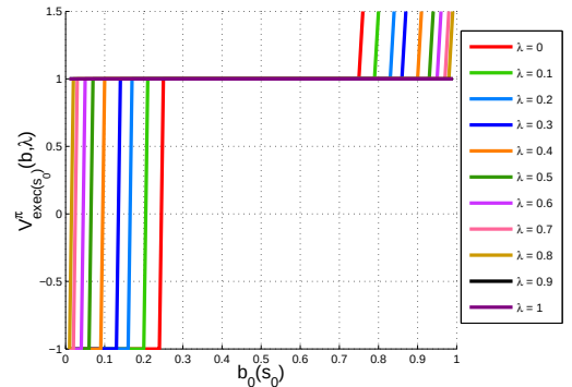
Figure 5: Rewards gathered at execution for different \lambda values depending on the agent's initial belief (which determines its policy) ; \lambda increases from inside to outside.
