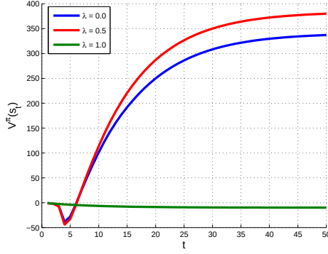
Figure 8: Value function of current state V^\pi(s_t) (averaged)
