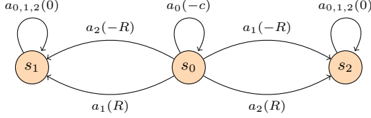
Figure 6: Counter example of entropy addition in criterion.
