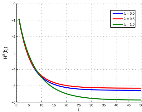
Figure 9: Cumulated weighted entropy of belief state H^\pi(b_t) (avg'd)
