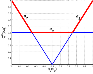
Figure 2: Q-values and value function (in bold) over b_0(s_0)
