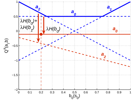
Figure 3: Q-value function for b_0(s_0) = 0.2 before(blue) and after(red) modification in the criterion.
