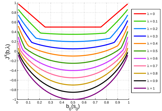
Figure 4: Best mixed-criterion based on the agent's initial belief for different \lambda values: \lambda increases from top curves to bottom ones.
