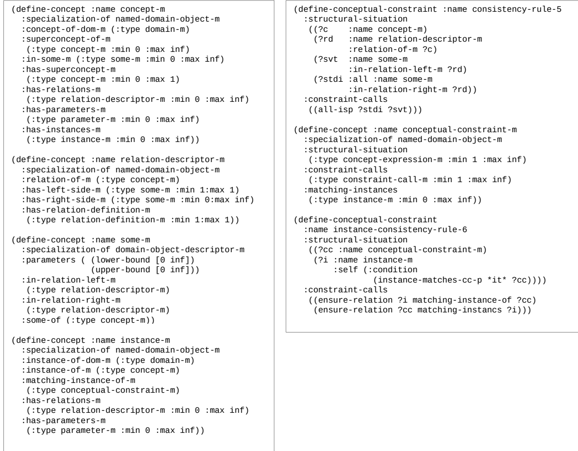
Figure 5. Formalizing the knowledge elements shown in Figure 4(a) and some consistency rules with CDL concepts.
