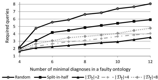
Figure 2. Number of queries required to select the target diagnosis D_t with threshold \sigma = 0.95 . Random and “split-in-half” are shown for |D_t| = 2 .
