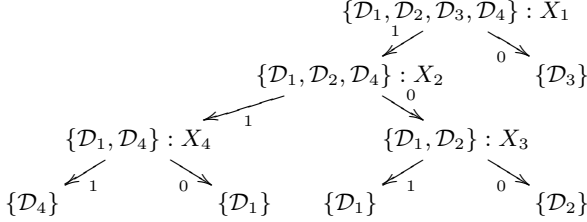
Figure 1. Greedy algorithm
