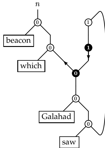
Figure 1.10: Graph after connecting all atomic formulas
