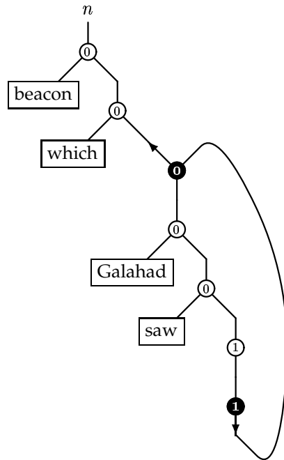
Figure 1.10: Graph after connecting all atomic formulas
