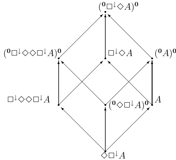
Figure 5.1: Some derivability patterns in \text{NL}(\Diamond, \cdot^0) .
