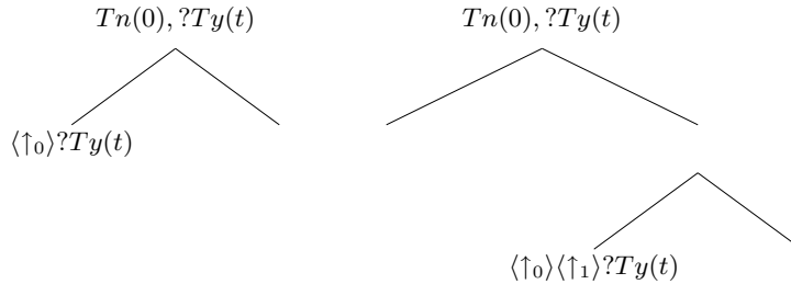
Figure 1.9: Proper and improper contexts for parsing they
