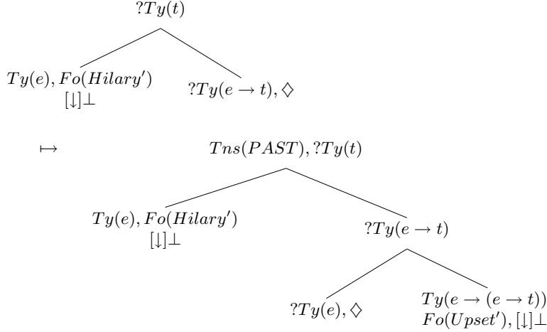
Figure 1.12: Parsing Hilary upset
