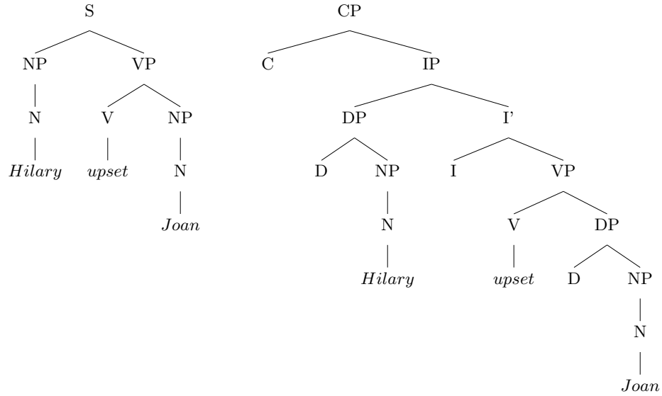
Figure 1.1: Representing the structure of strings
