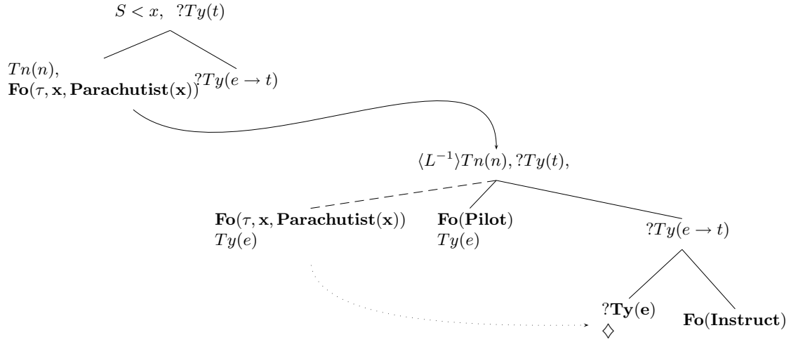
Figure 2.5: Parsing (2.29)
