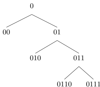
Figure 1.6: Tree Locations
