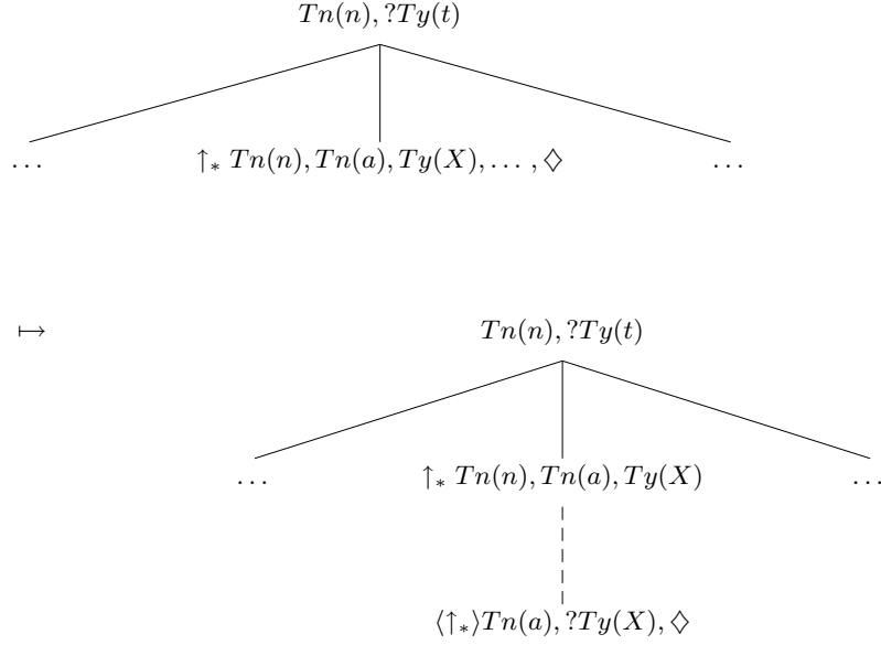
Figure 4.4: Late*Adjunction
