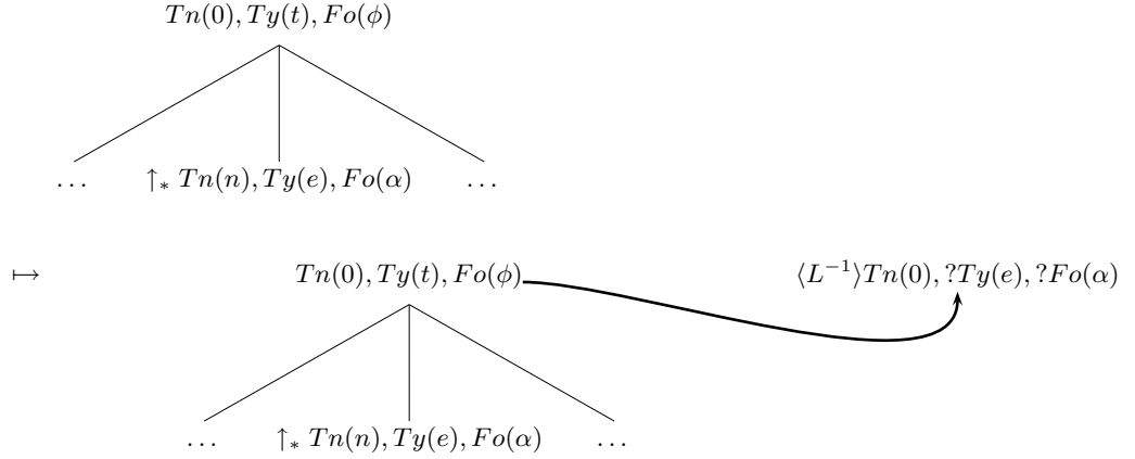
Figure 4.1: Licensing Recapitulation
