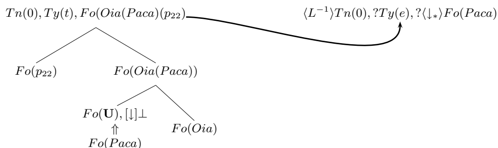
Figure 4.9: Parsing the accusative clitic
