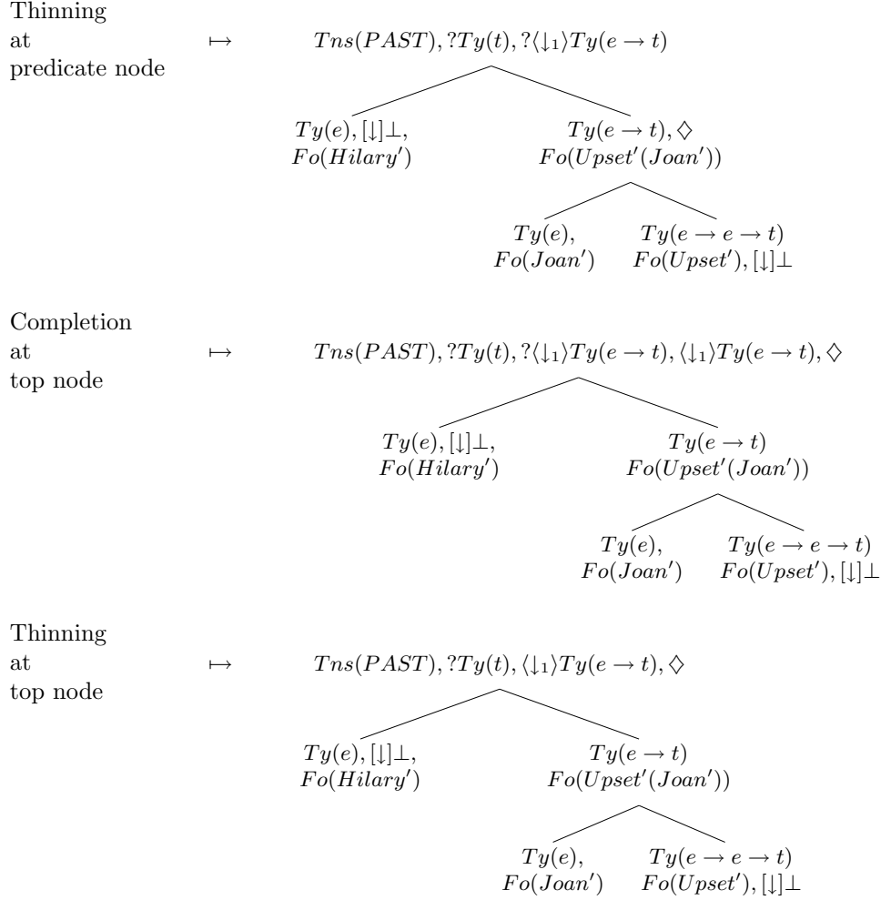
Figure 1.17: Moving the pointer to top-node in processing Hilary upset Joan
