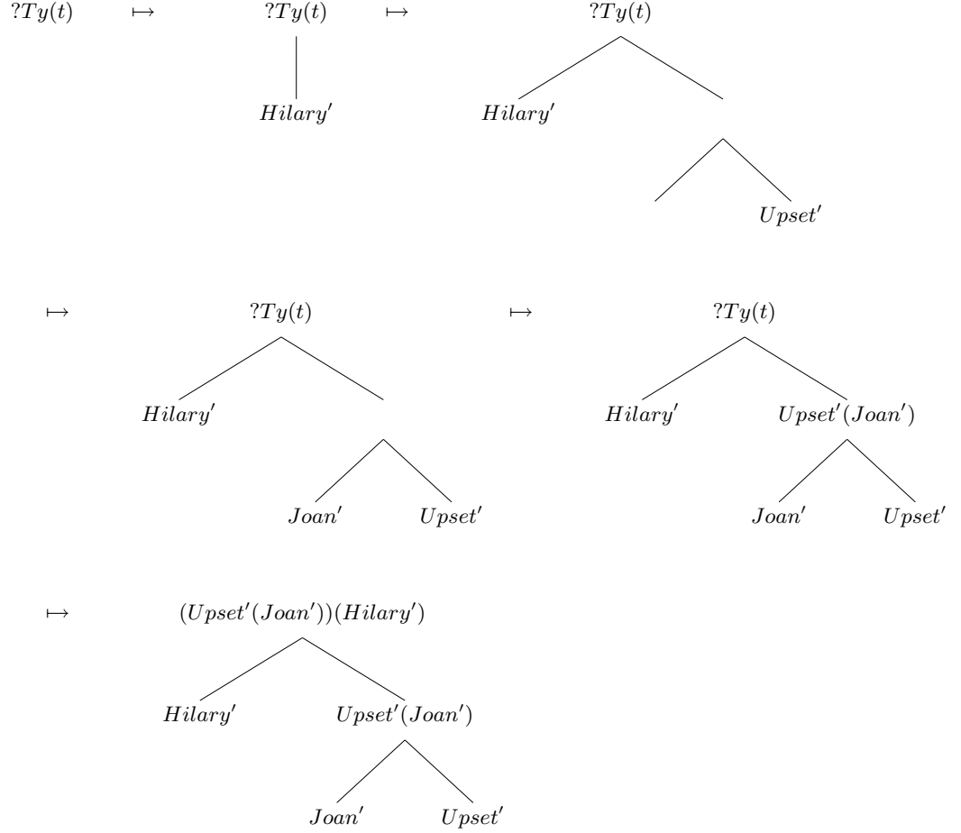
Figure 1.3: Parsing Hilary upset Joan
