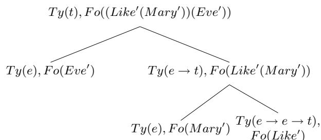
Figure 1.4: Representation of content of Eve likes Mary
