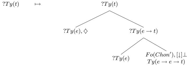
Figure 1.25: Parsing chonaic
