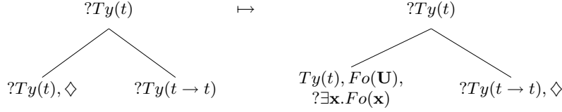
Figure 4.3: Parsing it
