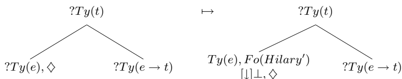
Figure 1.11: Parsing Hilary
