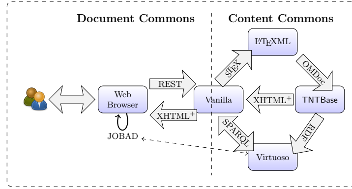
Fig. 5. The Planetary System Ecosystem
