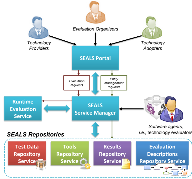
Fig. 1: Architecture of the SEALS Platform.
