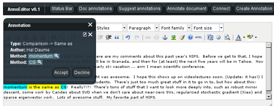
Fig. 2. Structure tag suggestions
