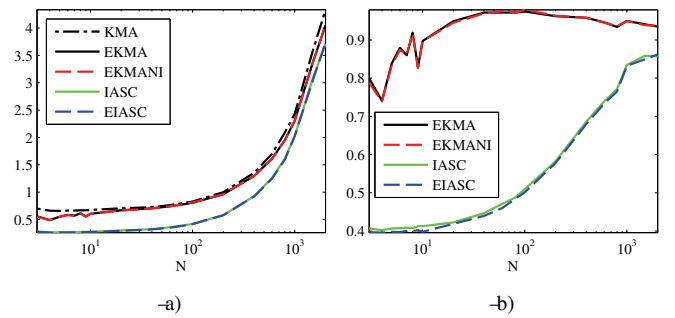
Fig. 2. –a) Total computation time (seconds) of the 1000 Monte Carlo simulations of uniformly distributed X_n and W_n , n = 1, 2, \dots, N for different N . –b) The ratio of the computation time of the four efficient algorithms with respect to KMA.
