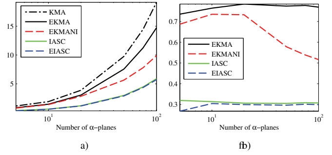
Fig. 4. (a) Total computation time (seconds) of the 1000 runs of centroid computation for different number of \alpha -planes. (b) The ratio of the computation time of the four efficient algorithms with respect to KMA.
