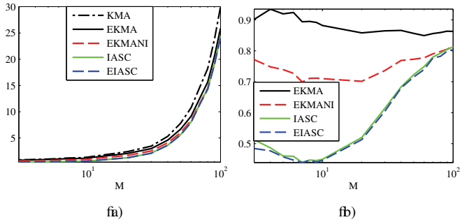
Fig. 11. (fa) Total computation time (seconds) of the 100 IT2 FLCs for different M , the number of IT2 FSs in each input domain. Note that N = M^2 . (fb) The ratio of the computation time of the efficient algorithms with respect to KMA.
