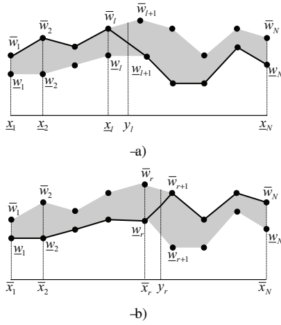
Fig. 1. Illustration of the switch points in computing l and r . -a) Computing l : switch from \bar{w}_l to \bar{w}_{l+1} -b) Computing r : switch from w_r to w_{r+1} .
