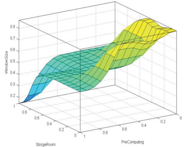
Figure 7: The output of the surface for the StorageRoom vs. PreComputing .
