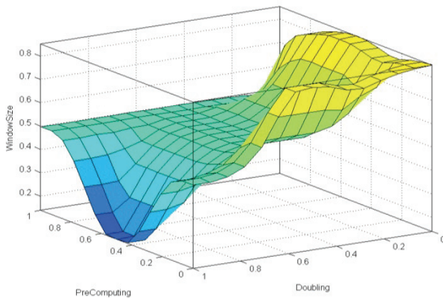
Figure 9: The output of the surface for the StorageRoom = constant (0.4) and PrecComputing vs. Doubling .
