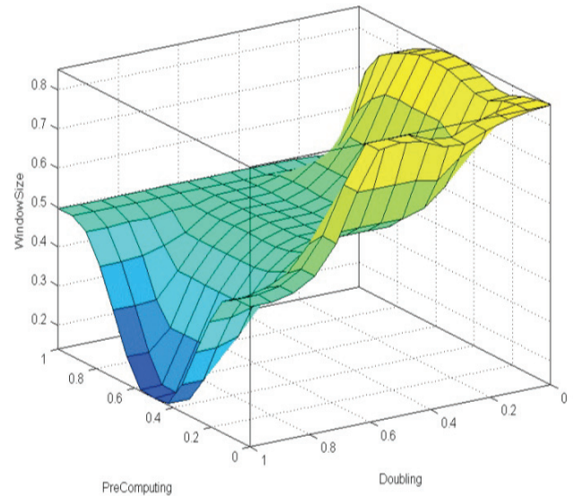
Figure 10: The output of the surface for the StorageRoom = constant (0.8) and PreComputing vs. Doubling .
