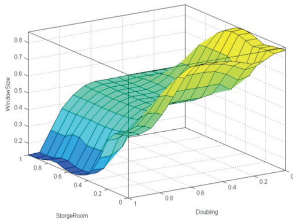
Figure 8: The output of the surface for the StorageRoom vs. Doubling .
