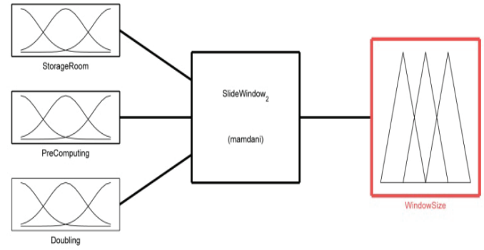
Figure 6: The block diagram of current fuzzy controller
