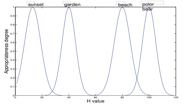
Fig. 4. Four image labels are predefined on the HSV space. This is the mapping of the labels on Hue (H) axis.
