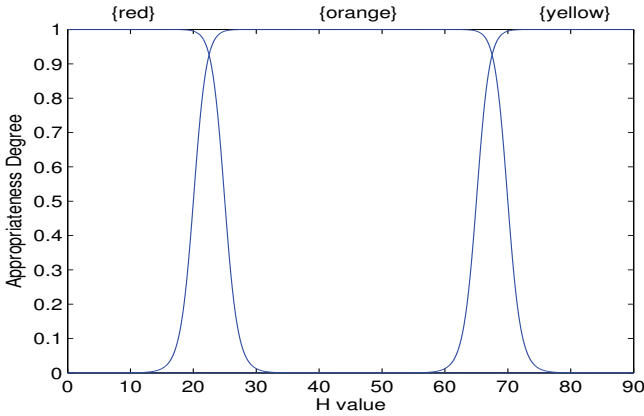
Fig. 3. Three linguistic labels: red (r), orange (o) and yellow (y). They are defined by bell-shape fuzzy sets on the Hue (H) values.
