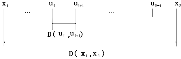
Fig. 1. Illustration of calculating the distance between two data points. The overall dissimilarity between \mathbf{x}_1 and \mathbf{x}_2 is the aggregated dissimilarity of all the neighboring points \mathbf{u}_i and \mathbf{u}_{i+1} for i \in R .
