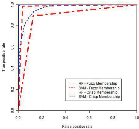
Figure 4. ROC curves for atherosclerosis prediction obtained using random forest (blue) and SVM (red)
