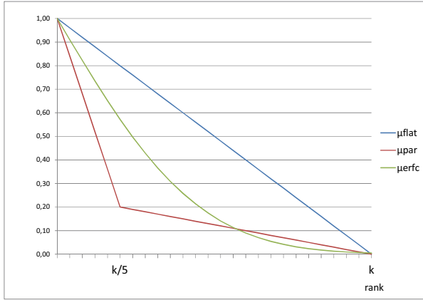
Figure 3 – Fuzzyfying functions
