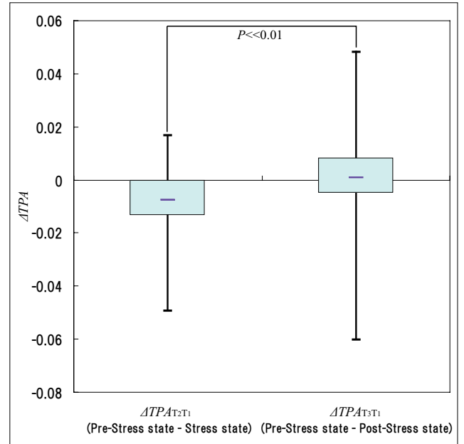
Fig. 13. Box plot of \Delta TPA . Paired t-test shows a significant differences at the 1% level between \Delta TPA_{T_2T_1} and \Delta TPA_{T_3T_1}
