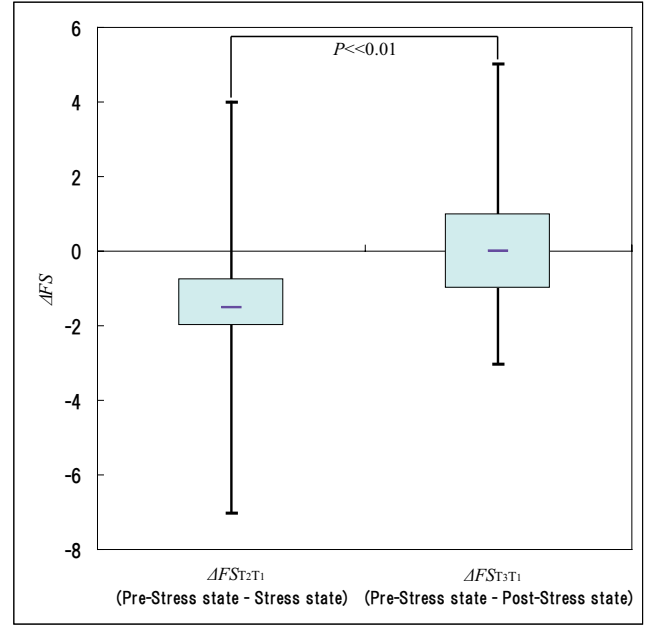
Fig. 12. Box plot of \Delta FS . Wilcoxon test shows a significant differences at the 1% level between \Delta FS_{T_2T_1} and \Delta FS_{T_3T_1}
