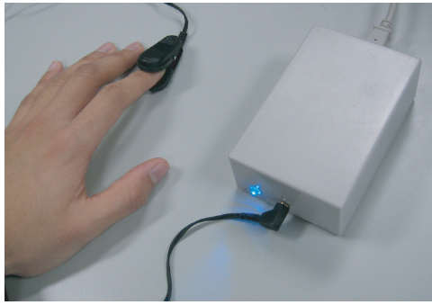
Fig. 1. Pulse sensor to measure finger plethysmogram
