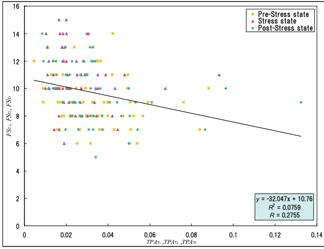
Fig. 8. Scatter plot of TPA_f and FS
