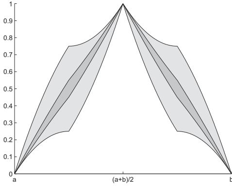
Fig. 2: Ignorance weighting factor genetic tuning. The final values of the parameters are: \delta = 0.1 , \gamma = 0.1 .
