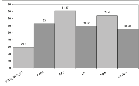
Fig. 3: Rankings of the different fuzzy decision trees.
