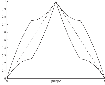
Fig. 1: Initial constructed IVFS.
