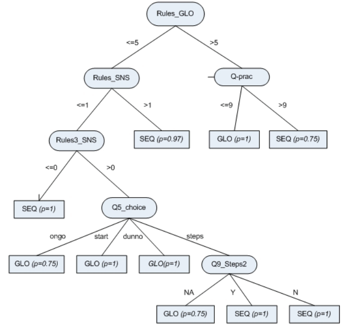
Fig. 3. Crisp tree representing sequential-global dimension
