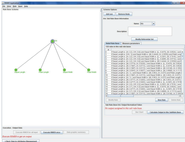
Figure 8. Main window with Iris problem structure defined
