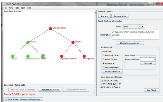
Figure 1 (b) Hierarchical structure window as main window
