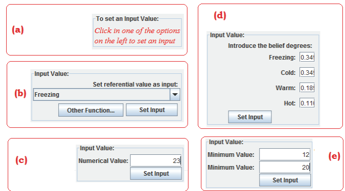
Figure 4. Different inputs that can be assigned
