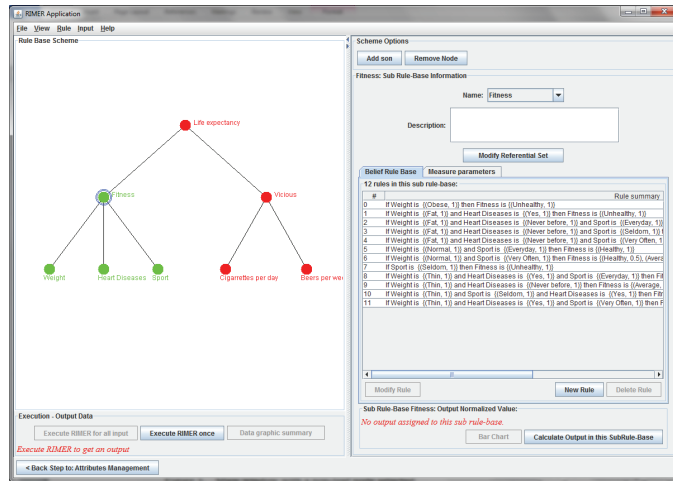
Figure 3. Main window with a non-leaf node selected
