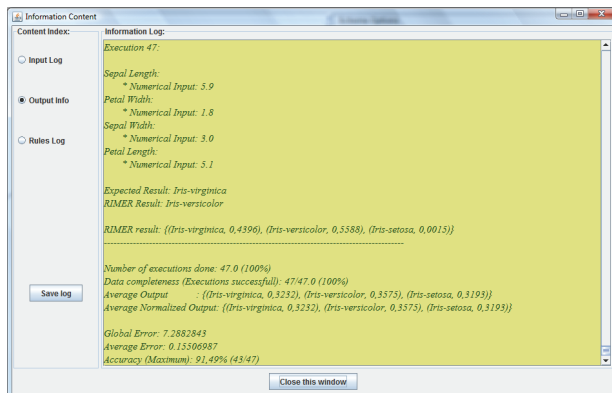
Figure 6. Statistics of the multi-execution mode for the Iris data set
