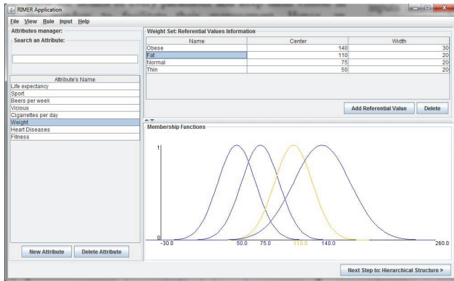
Figure 1 (a) Attribute window
