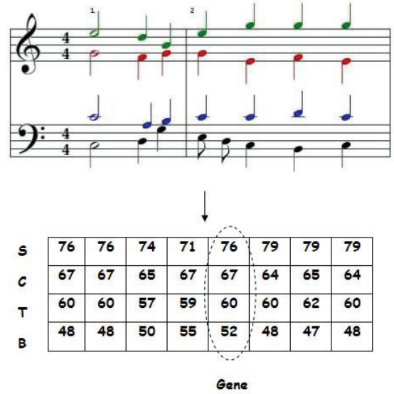
Fig. 4. Chromosome and MIDI representation
