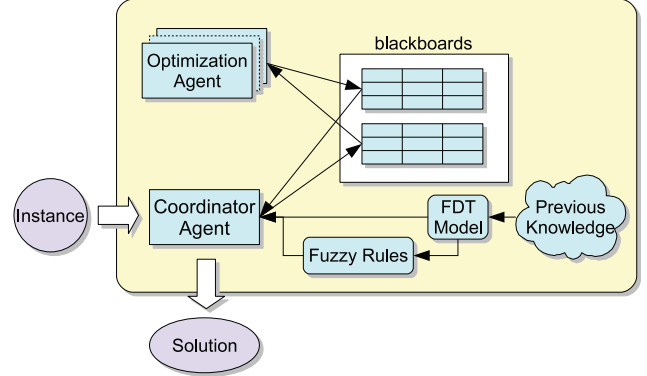
Fig. 2. Architecture of the cooperative metaheuristic strategy
