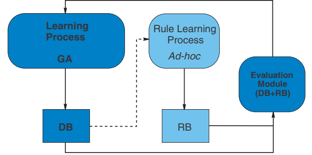
Fig. 4. Learning scheme of the KB
