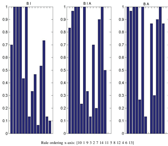
Fig. 1. Selected Rules for MOEA in PLA1
