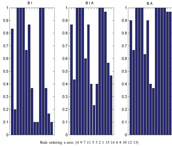
Fig. 3. Selected Rules for MOEA in STP1
