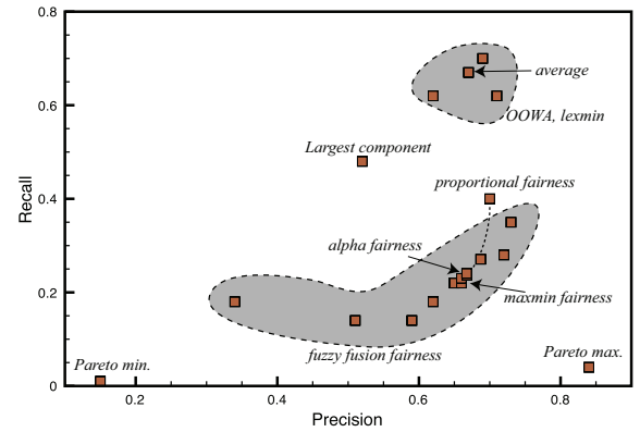
Fig. 3. Precision vs. Recall for the used relations.
