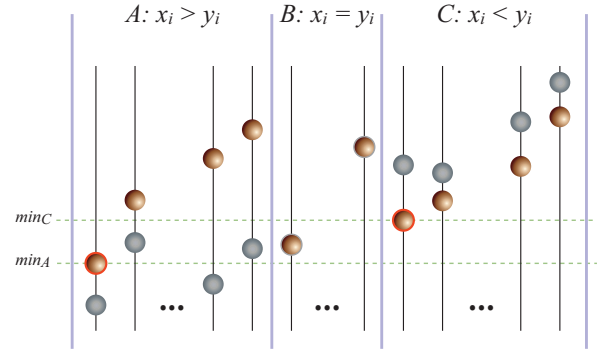
Fig. 2. Maxmin fairness relation can be more easily defined, if we consider the sets of components of x larger (set A ) and smaller (set C ) than corresponding components of y . Vector x will maxmin fair dominate y if and only if the smallest larger component of x is smaller than or equal to the smallest smaller component of x [5]. In the figure, corresponding components of x and y are placed on the same line, with height indicating their magnitude, and the lines are re-arranged to show first x -components larger than the corr. y -component, then equal components, and third smaller components (each of the three sections are additionally arranged by increasing size of the corr. x -component).
