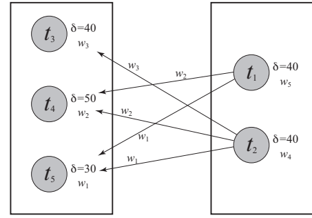
Fig. 4. Example for the bi-graph used in the proof.
