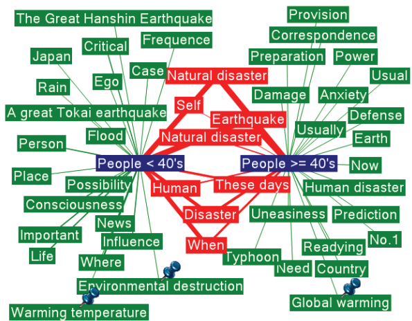
Fig. 4. Conventional HK Graph (Bases : People < 40 's, People \geq 40 's)
