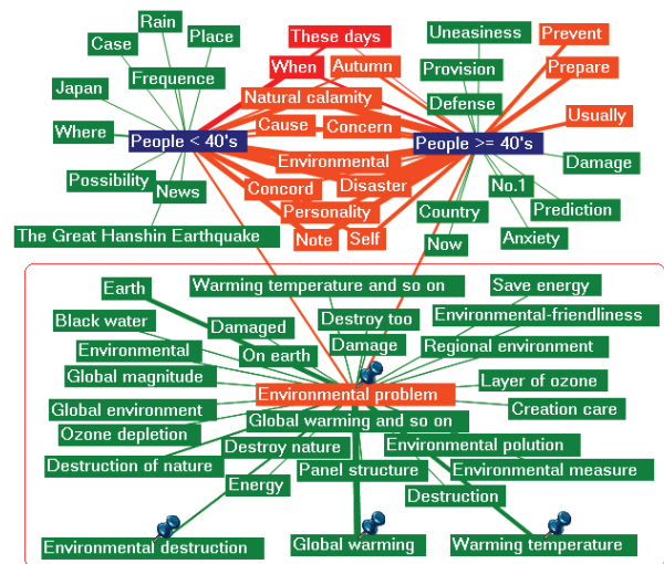
Fig. 4. Conventional HK Graph (Bases : People < 40 's, People \geq 40 's)
