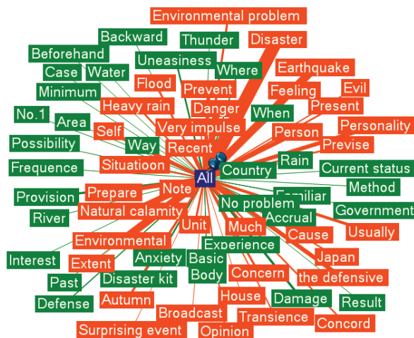
Fig. 3. Proposed method
