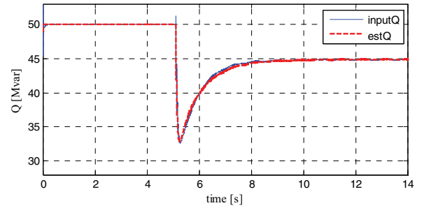
Figure 11. Load model response (reactive power)
