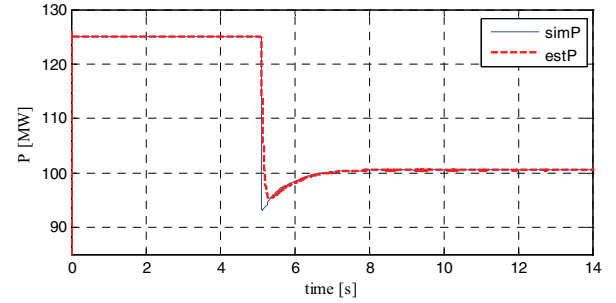
Figure 5. Simulated P versus estimated P
