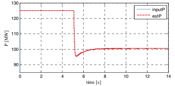
Figure 10. Load model response (active power)
