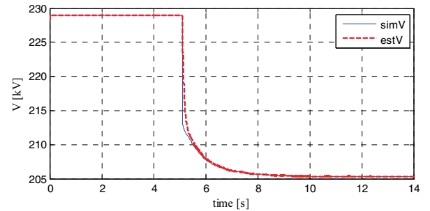
Figure 7. Simulated V versus estimated V
