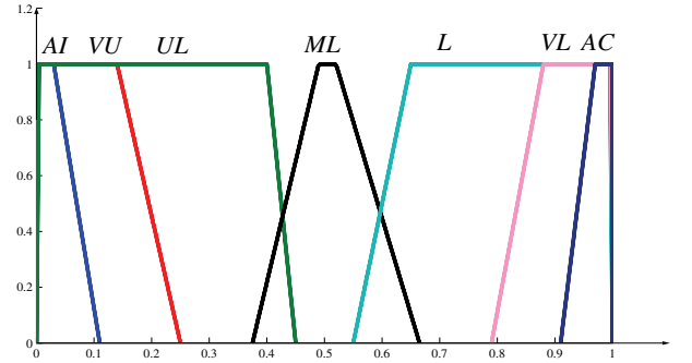
Fig. 2. The membership functions of the vocabulary of type-1 linguistic probabilities.
