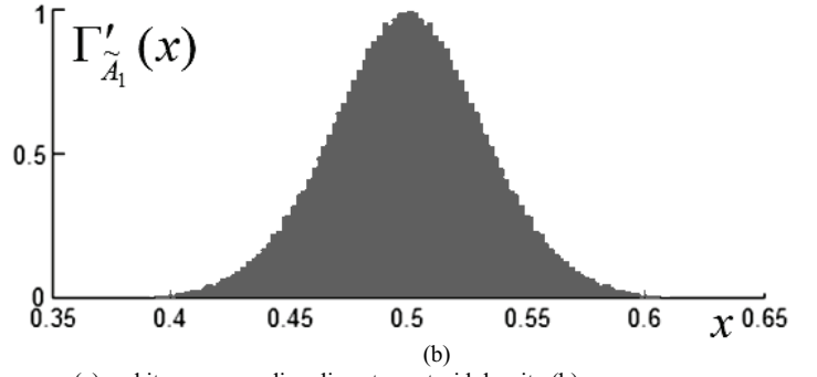
Fig. 1 Interval Type-2 Gaussian fuzzy set with uncertain mean (a) and its corresponding discrete centroid density (b).
