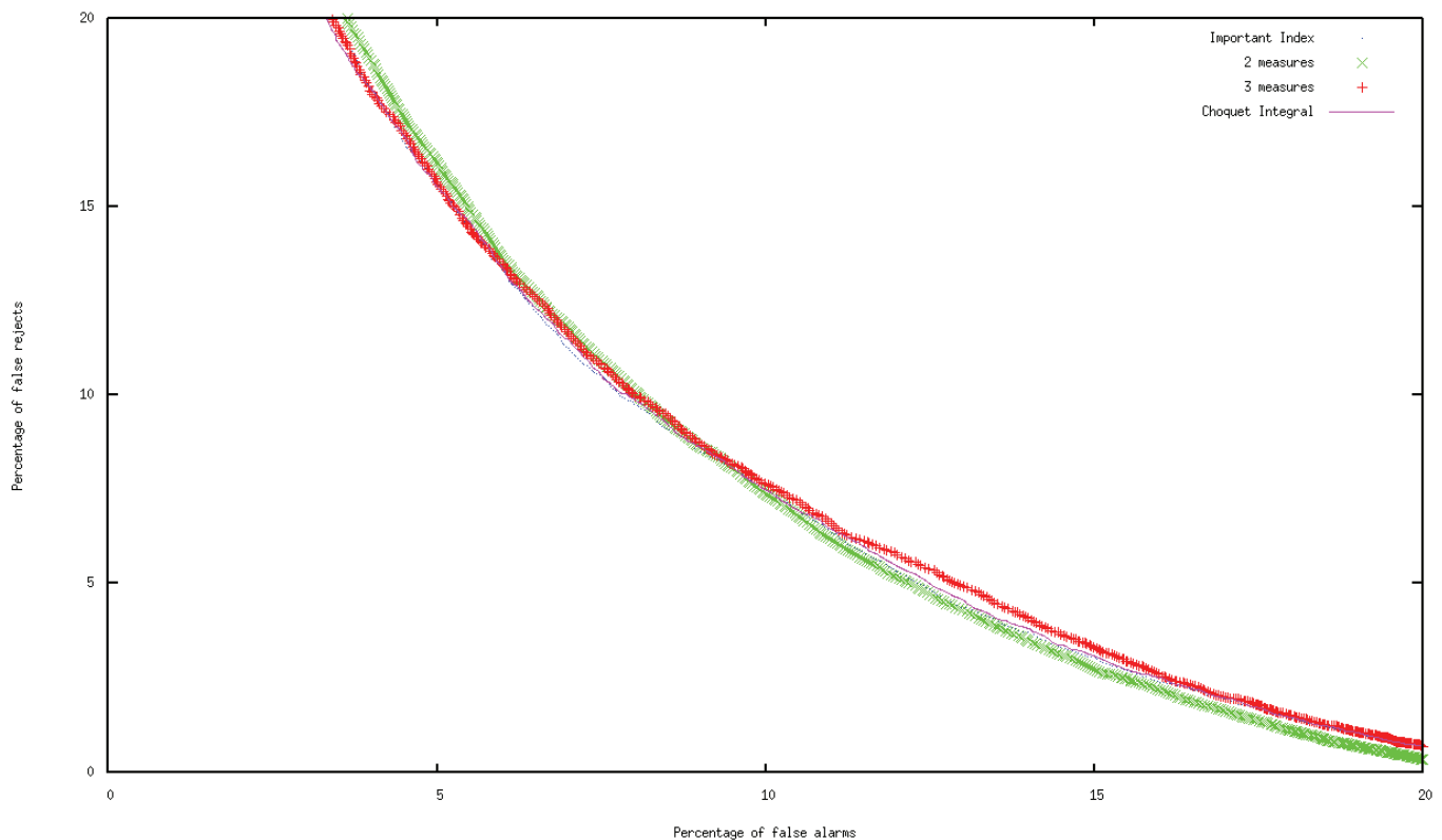
Fig. 2. DET curve for the Choquet Integral with 4, 3 and 2 measures and with the linear regression with important indexes.
