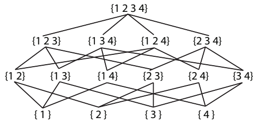
Fig. 1. Lattice for 4 measures. Each path is associated with a weight processed by the Choquet Integral technique on MTrain. {1}, {2}, {3}, {4} corresponds respectively to the weights associated to the WP, MAP, AC and LMBB measure.
