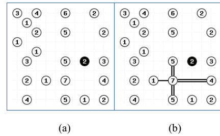
Figure 5. An example of first kind of sieving
