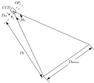
Figure 2. The internal parameters diagram of a CCD camera. By the theorem of similar triangles, D_{OP} can be found as shown in (2) and (3).
