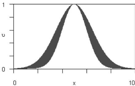
Figure 7 An example of a Gaussian interval type-2 membership function produced using the R toolkit.
