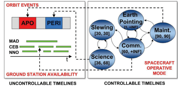
Figure 3: MrSPOCK domain model
