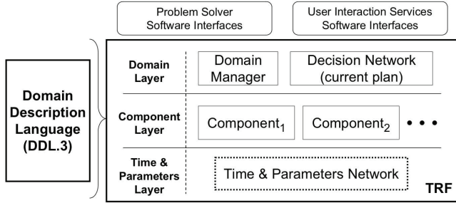
Figure 1: The layered implementation of the TRF
