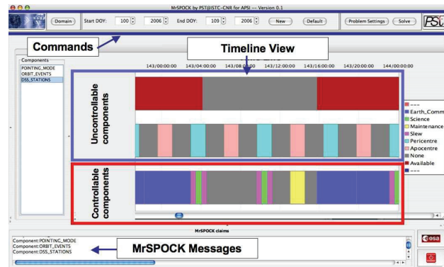
Figure 4: Basic interaction layout
