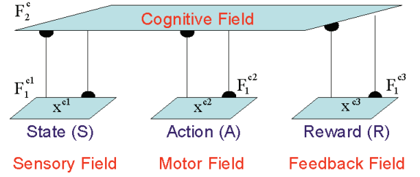
Figure 1: FALCON architecture.
