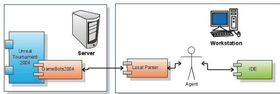
Figure 3: Pogamut architecture.
