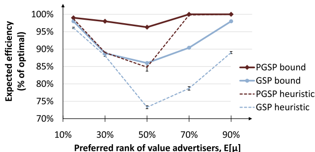
Figure 4: The value of our upper bound on expected efficiency and the efficiency of the heuristic bidding strategy for the GSP and PGSP mechanisms. Large values of E[\mu] correspond to runs in which higher ranking positions are more valuable for the value advertisers and vice versa.
