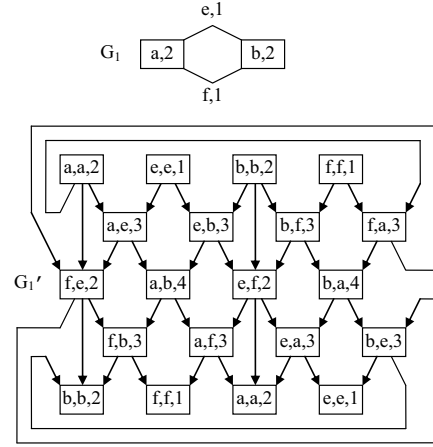
Figure 2: First Example for Theorem 9
