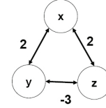
Figure 2: An affinity graph for which the coalitional affinity game has an empty core.
